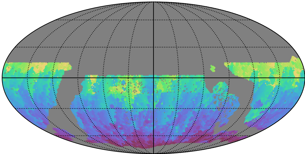
too_combined_s0.5_v3.4_10yrs WFD g band: Min HA
