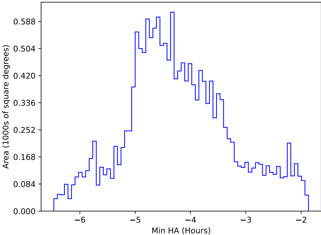
too_combined_s0.5_v3.4_10yrs WFD g band: Min HA
