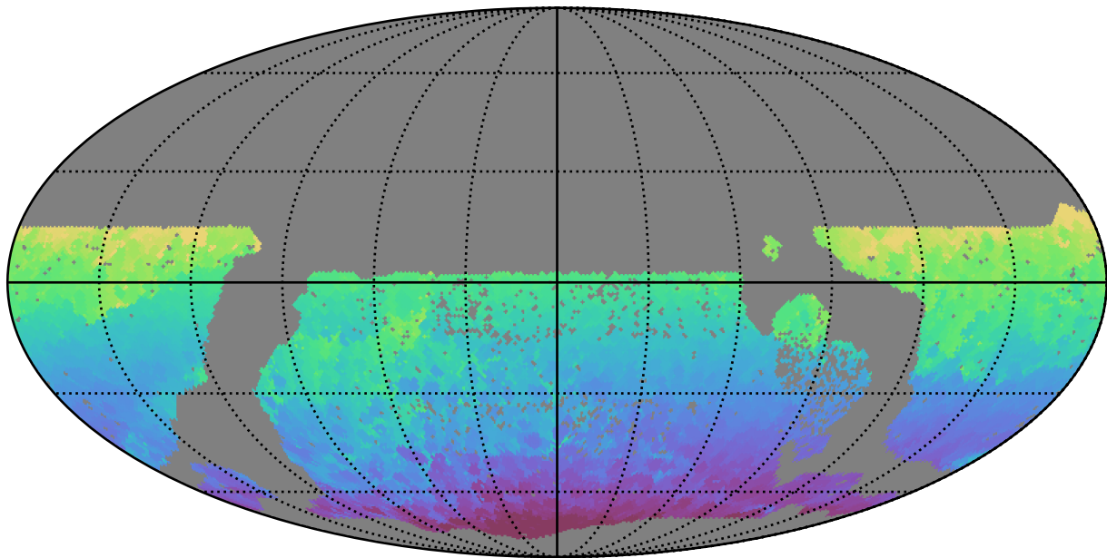
too_combined_s0.5_v3.4_10yrs WFD all bands: Min HA
