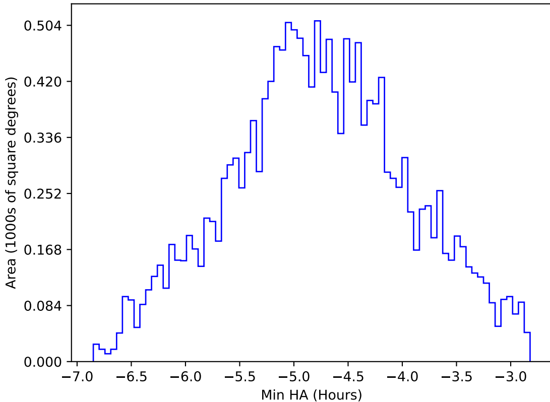
too_combined_s0.5_v3.4_10yrs WFD all bands: Min HA
