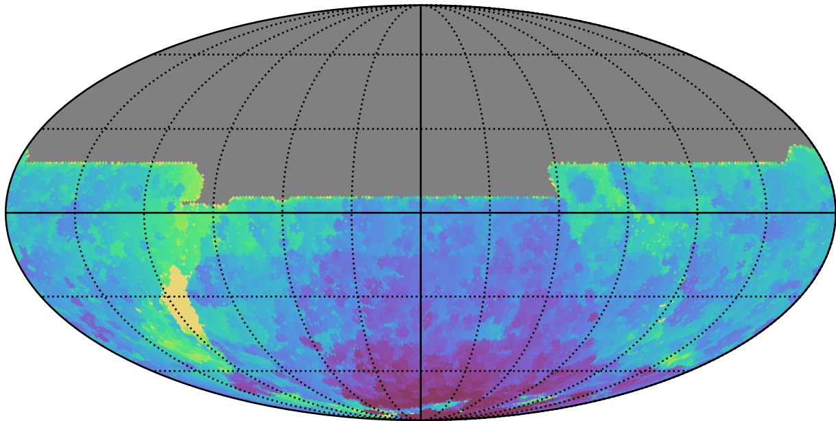
too_combined_s0.5_v3.4_10yrs All sky y band: Min HA
