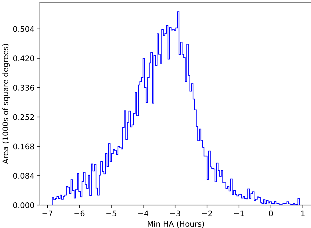
too_combined_s0.5_v3.4_10yrs All sky y band: Min HA
