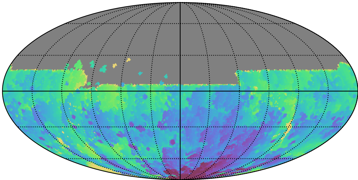
too_combined_s0.5_v3.4_10yrs All sky u band: Min HA
