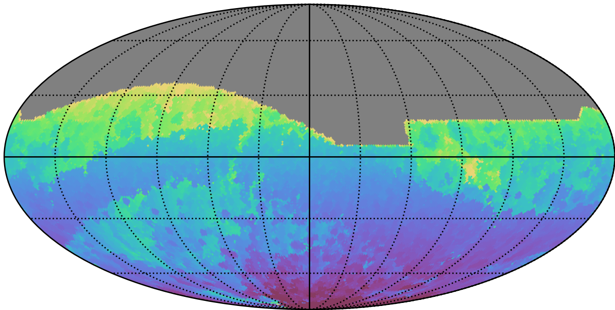
too_combined_s0.5_v3.4_10yrs All sky r band: Min HA
