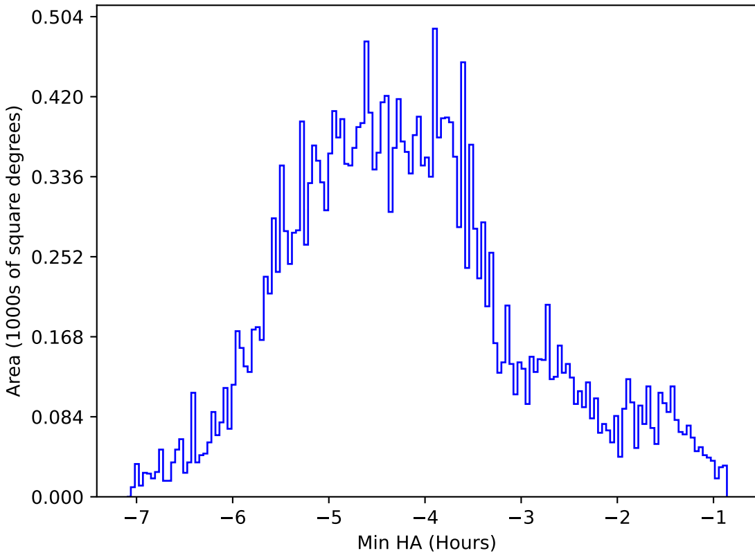
too_combined_s0.5_v3.4_10yrs All sky r band: Min HA
