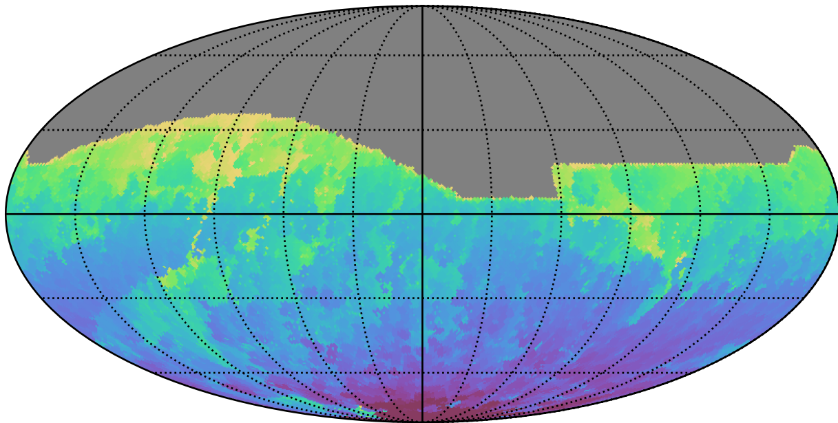
too_combined_s0.5_v3.4_10yrs All sky i band: Min HA
