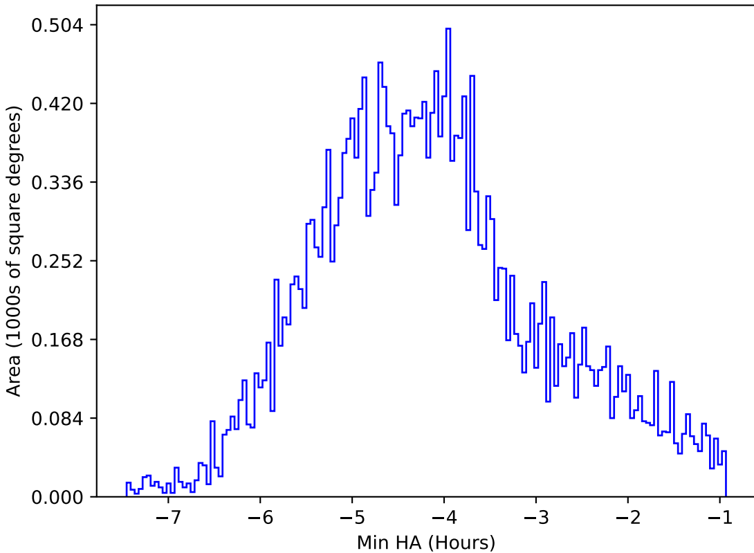
too_combined_s0.5_v3.4_10yrs All sky i band: Min HA
