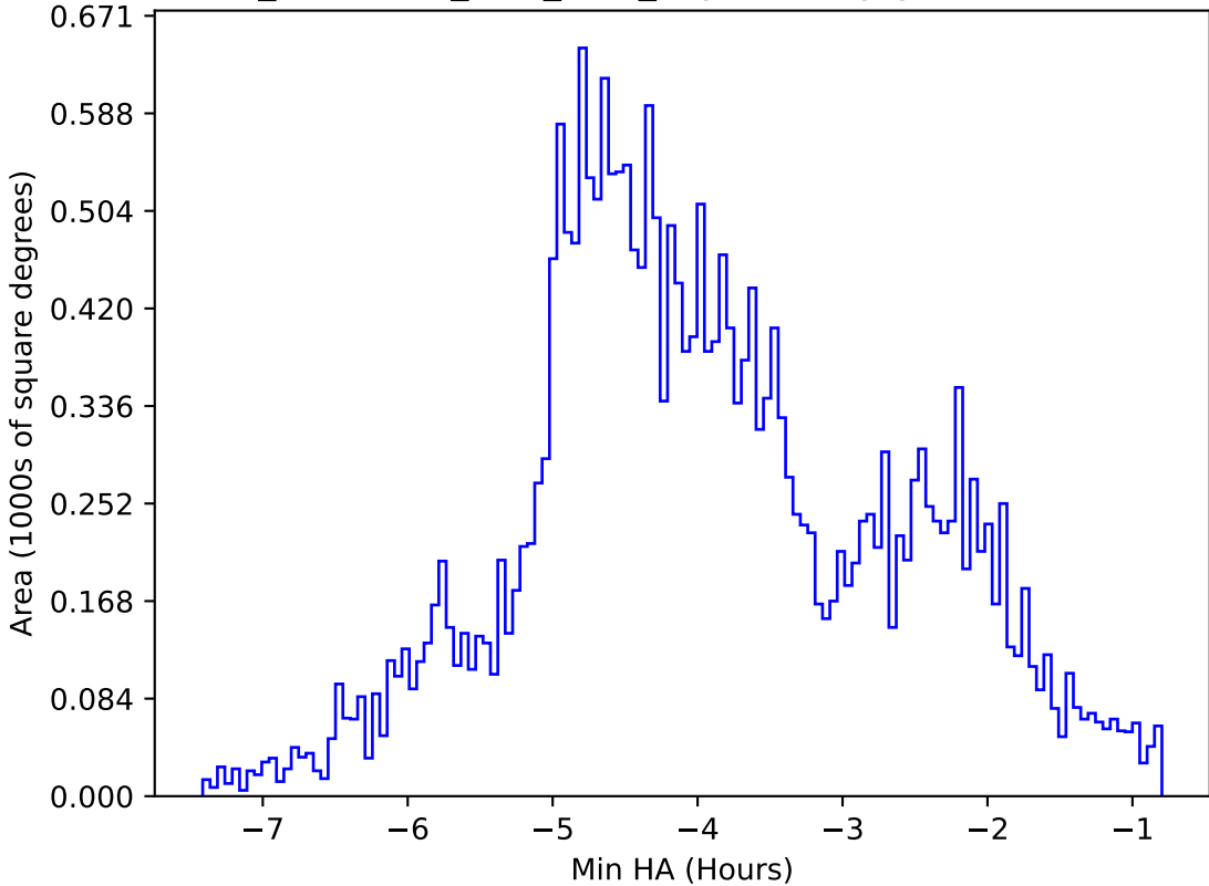
too_combined_s0.5_v3.4_10yrs All sky g band: Min HA
