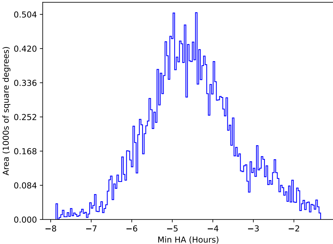
too_combined_s0.5_v3.4_10yrs All sky all bands: Min HA
