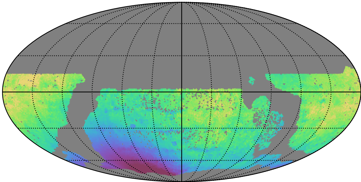
too_combined_s0.5_v3.4_10yrs WFD z band: Median solarElong
