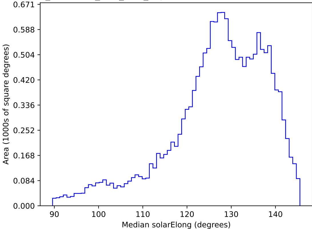
too_combined_s0.5_v3.4_10yrs WFD z band: Median solarElong
