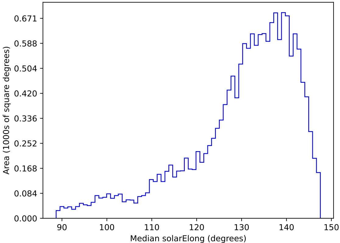
too_combined_s0.5_v3.4_10yrs WFD y band: Median solarElong
