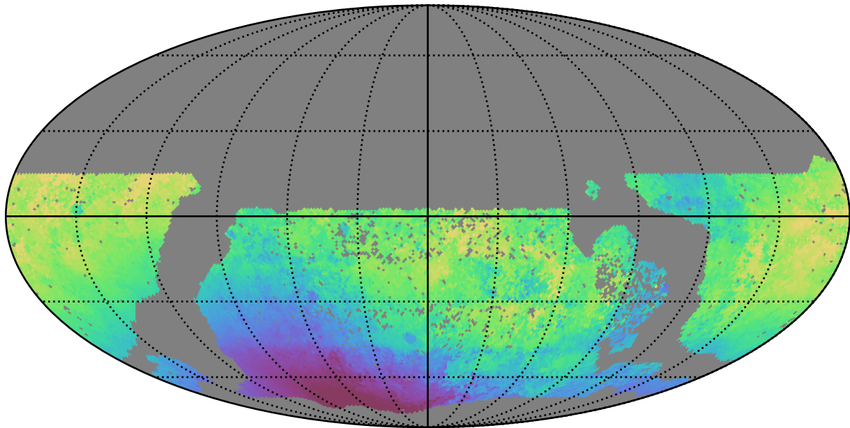
too_combined_s0.5_v3.4_10yrs WFD u band: Median solarElong
