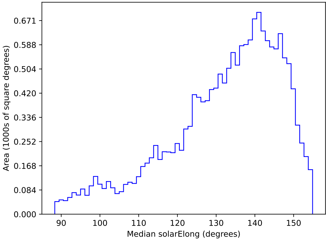
too_combined_s0.5_v3.4_10yrs WFD u band: Median solarElong
