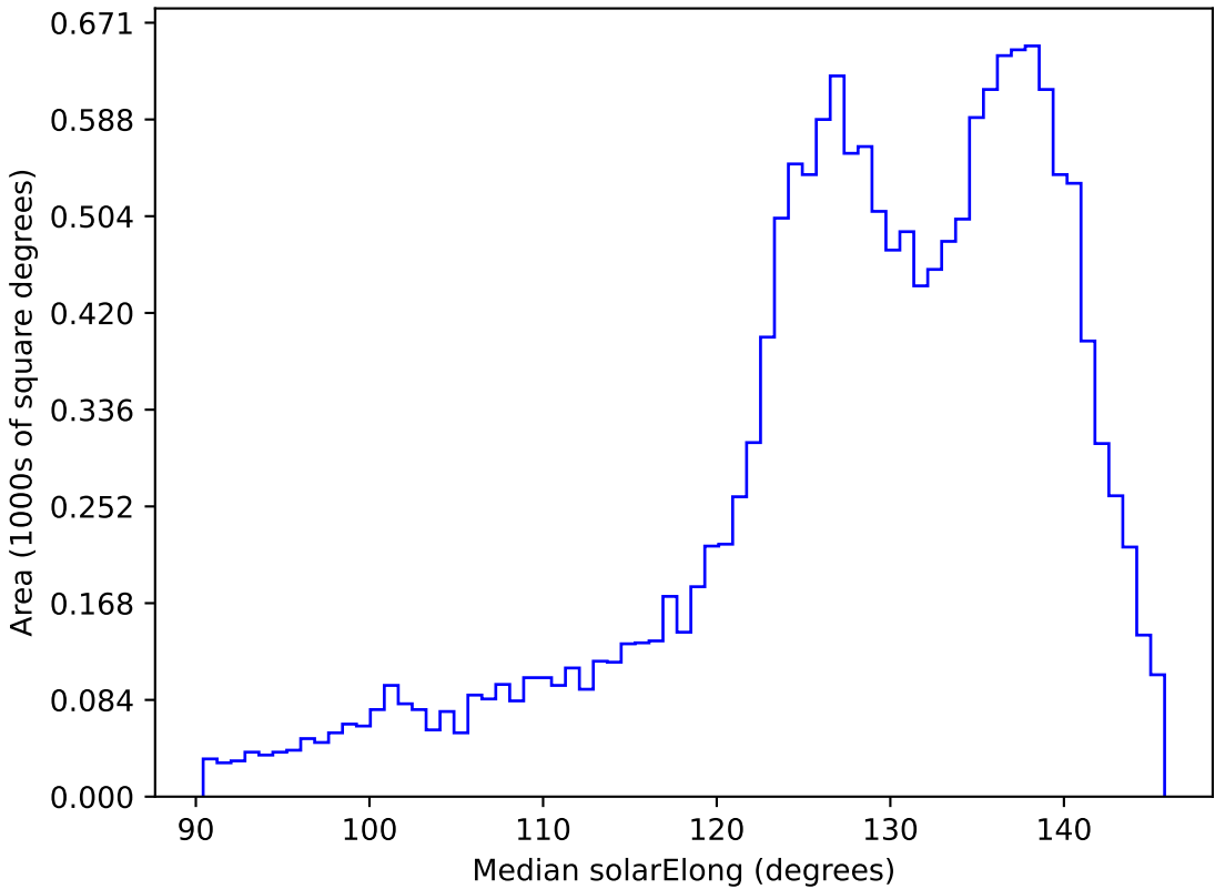
too_combined_s0.5_v3.4_10yrs WFD i band: Median solarElong
