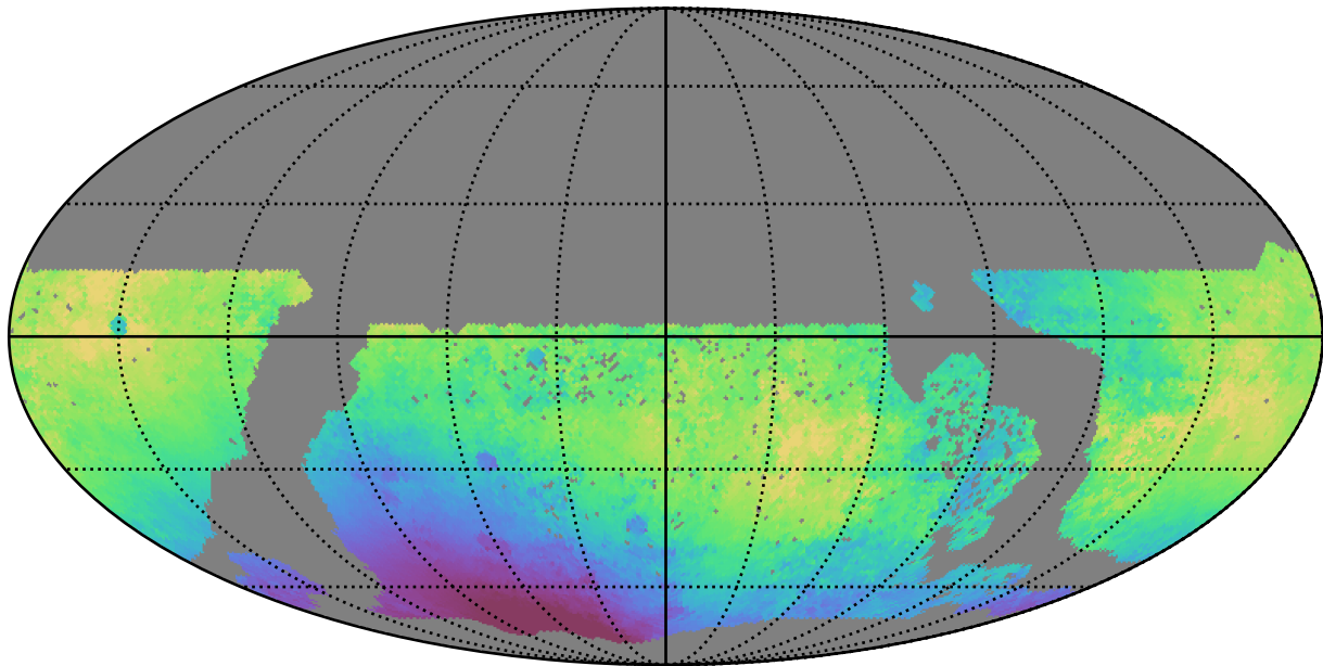
too_combined_s0.5_v3.4_10yrs WFD g band: Median solarElong
