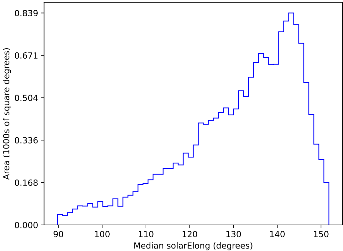
too_combined_s0.5_v3.4_10yrs WFD g band: Median solarElong
