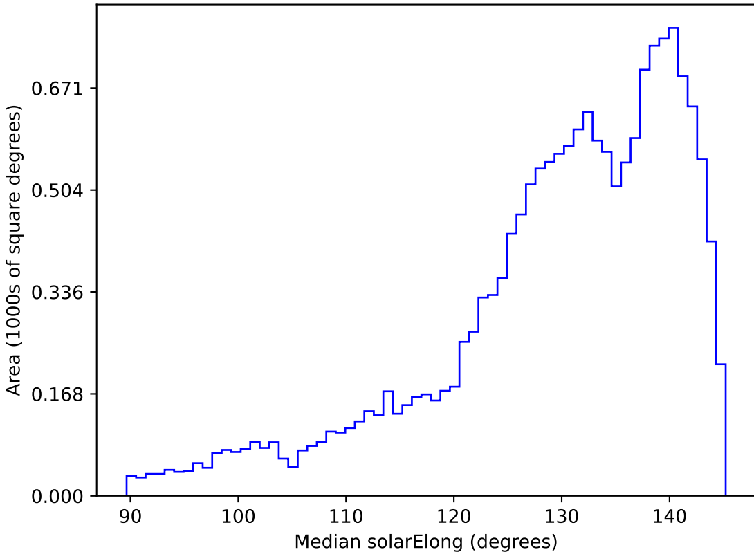
too_combined_s0.5_v3.4_10yrs WFD all bands: Median solarElong
