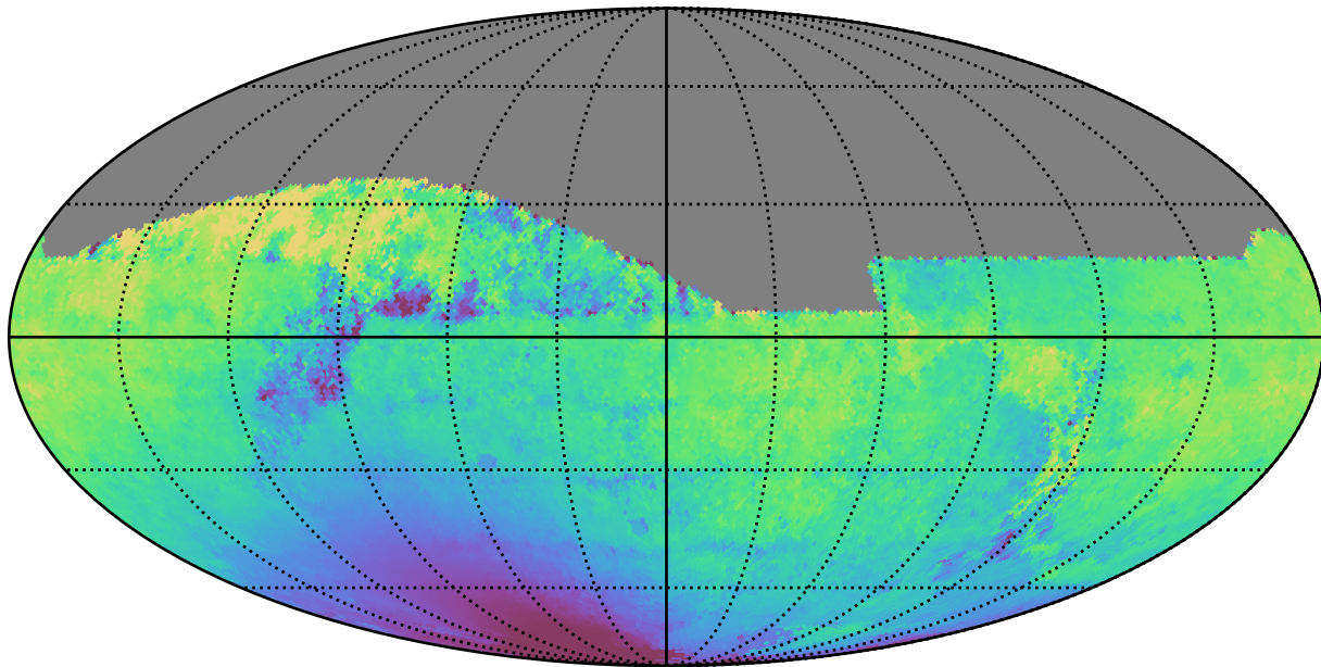
too_combined_s0.5_v3.4_10yrs All sky z band: Median solarElong
