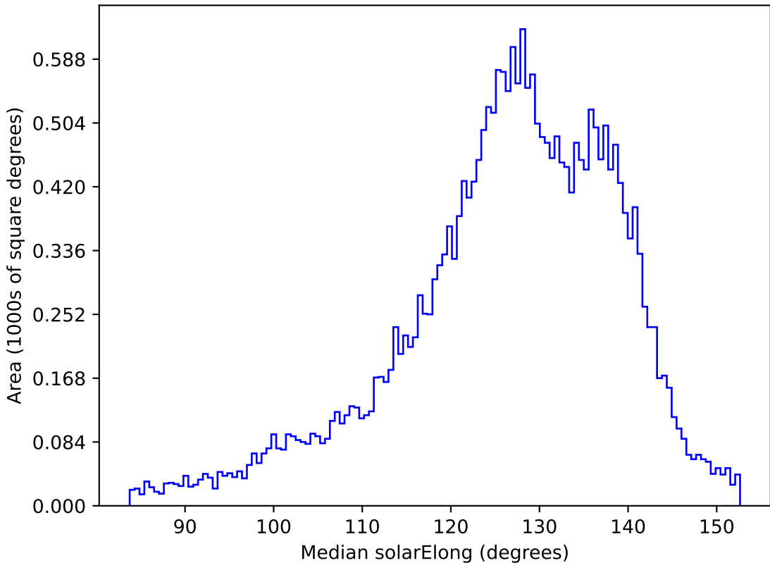
too_combined_s0.5_v3.4_10yrs All sky z band: Median solarElong
