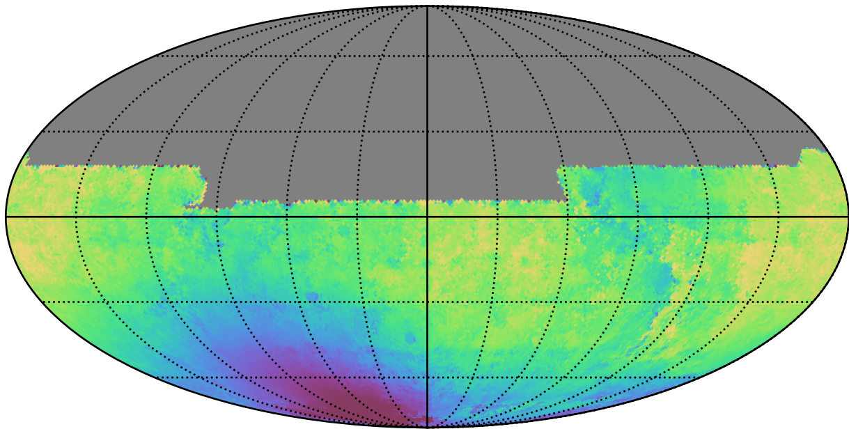
too_combined_s0.5_v3.4_10yrs All sky y band: Median solarElong
