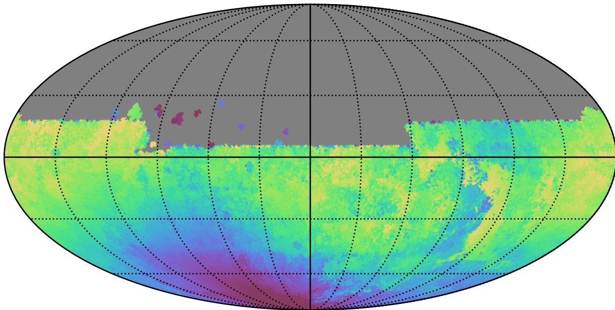
too_combined_s0.5_v3.4_10yrs All sky u band: Median solarElong
