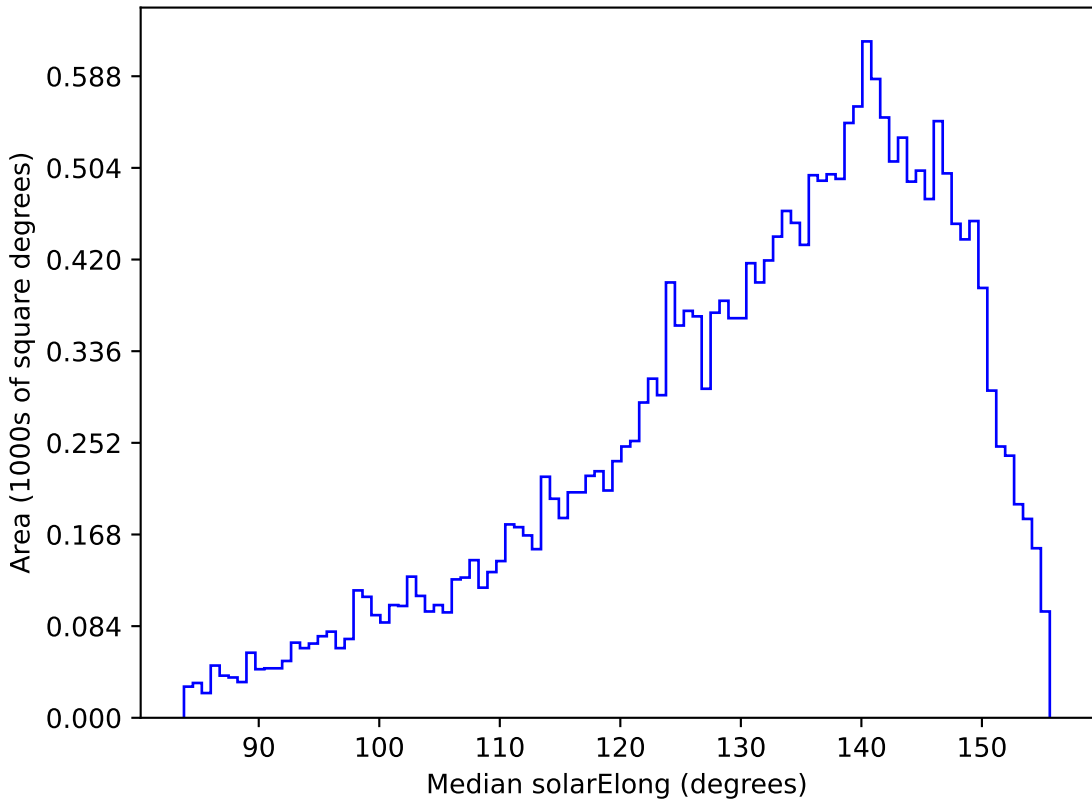
too_combined_s0.5_v3.4_10yrs All sky u band: Median solarElong
