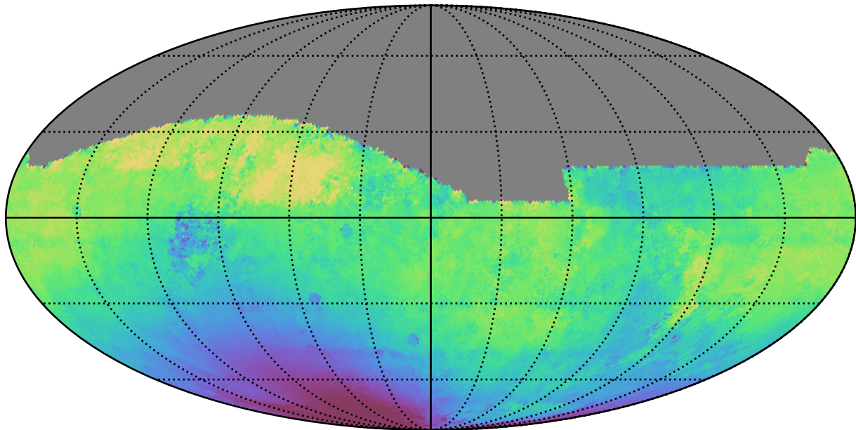
too_combined_s0.5_v3.4_10yrs All sky r band: Median solarElong
