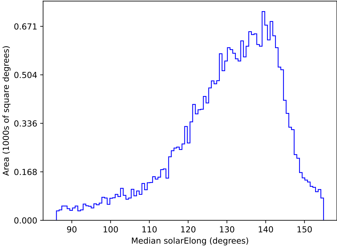
too_combined_s0.5_v3.4_10yrs All sky r band: Median solarElong
