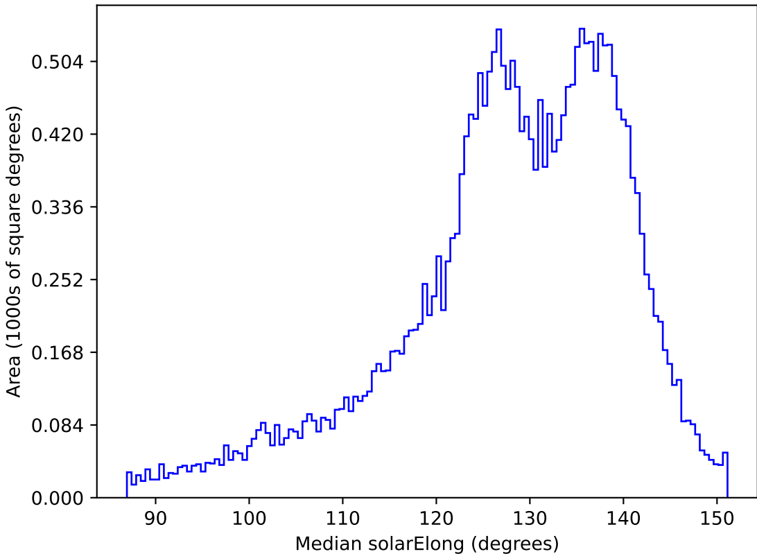
too_combined_s0.5_v3.4_10yrs All sky i band: Median solarElong
