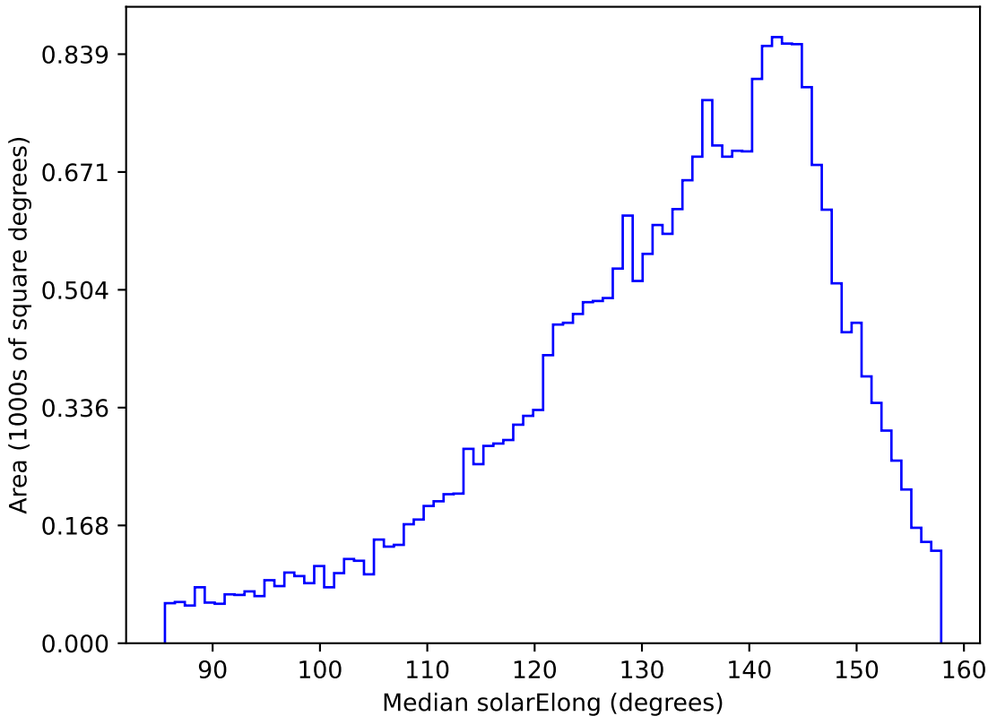
too_combined_s0.5_v3.4_10yrs All sky g band: Median solarElong
