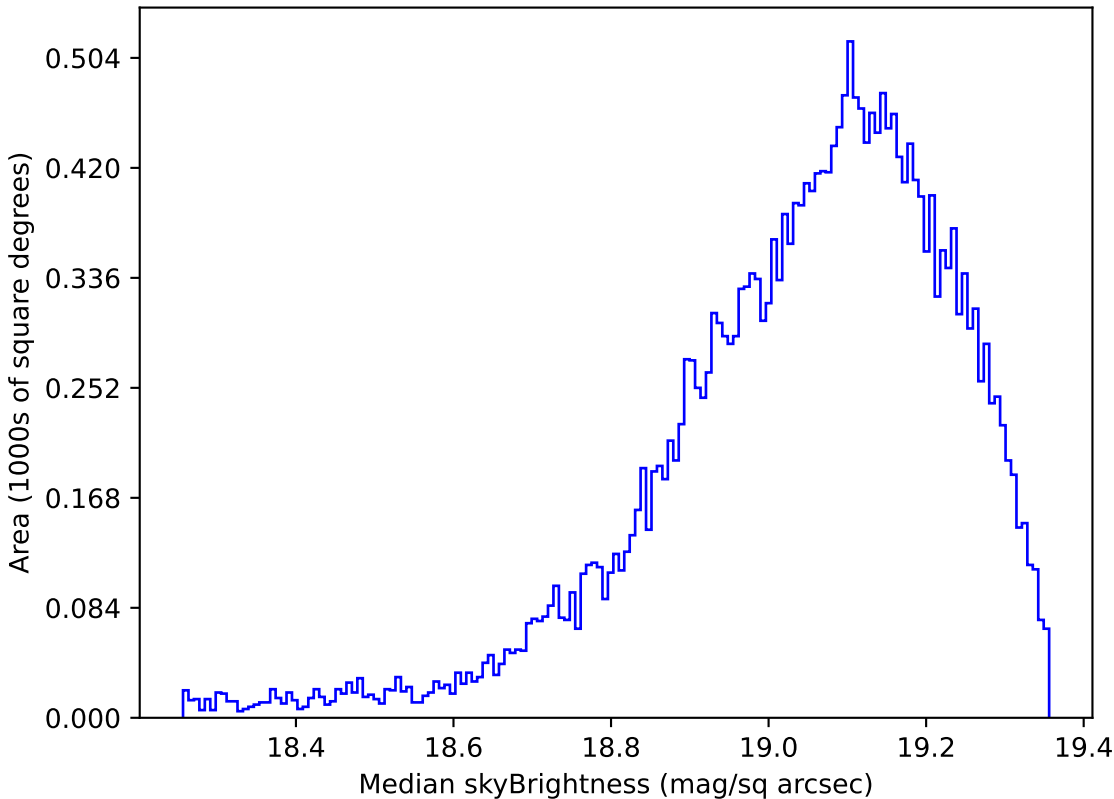
too_combined_s0.5_v3.4_10yrs Yr 1 z band: Median skyBrightness
