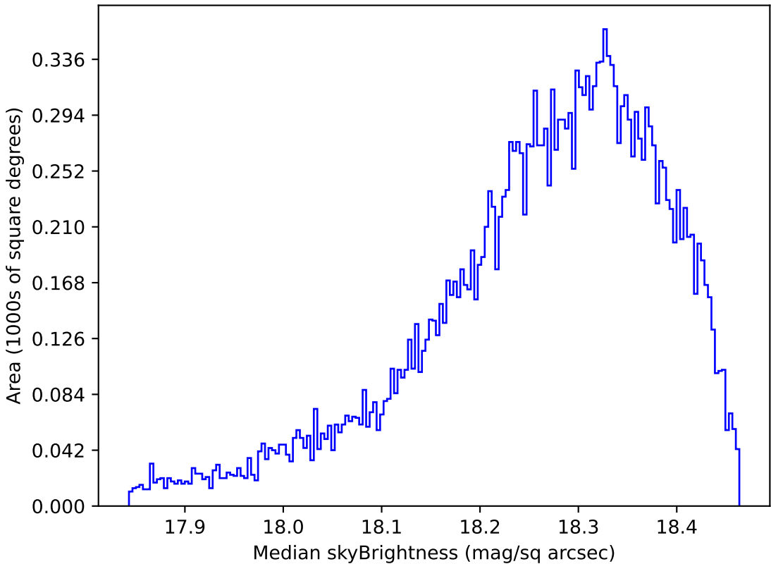
too_combined_s0.5_v3.4_10yrs Yr 1 y band: Median skyBrightness
