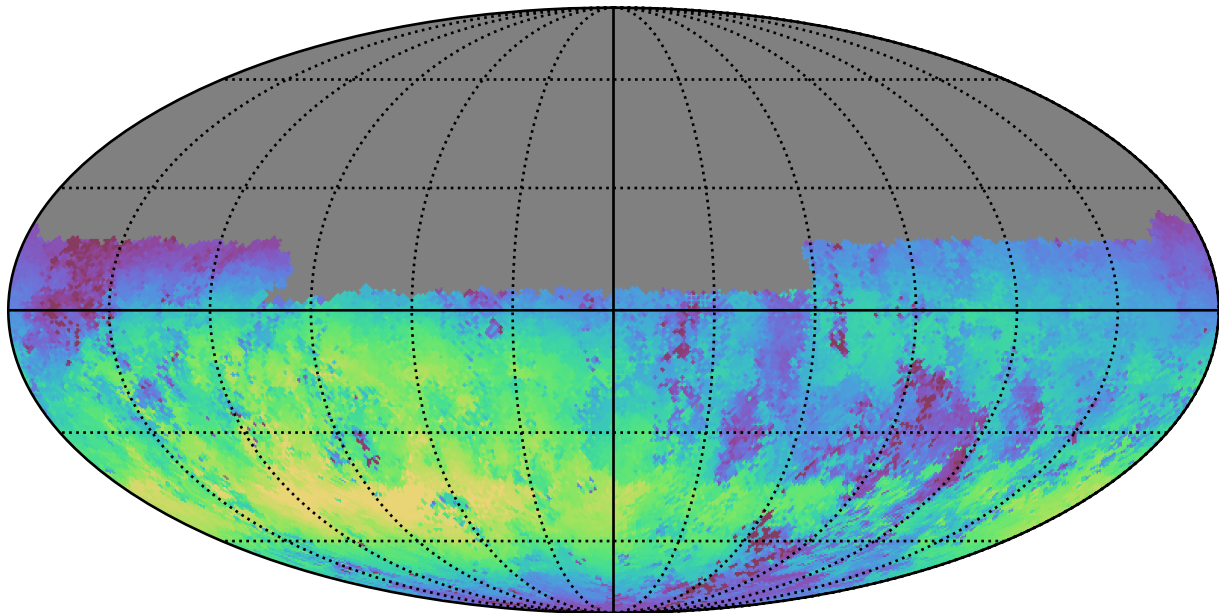
too_combined_s0.5_v3.4_10yrs Yr 1 u band: Median skyBrightness
