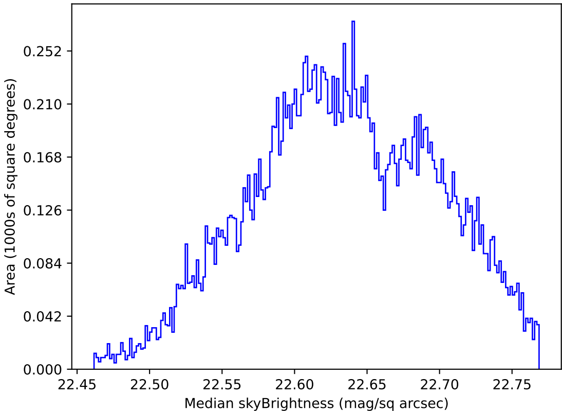
too_combined_s0.5_v3.4_10yrs Yr 1 u band: Median skyBrightness
