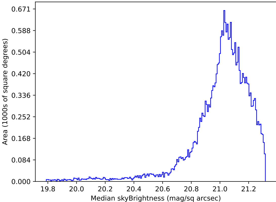
too_combined_s0.5_v3.4_10yrs Yr 1 r band: Median skyBrightness
