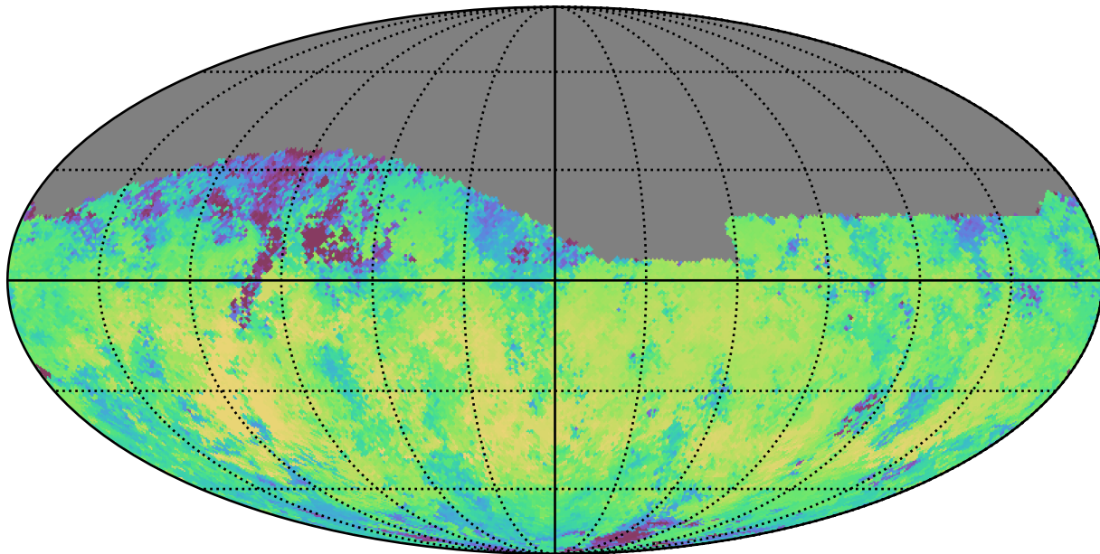
too_combined_s0.5_v3.4_10yrs Yr 1 i band: Median skyBrightness
