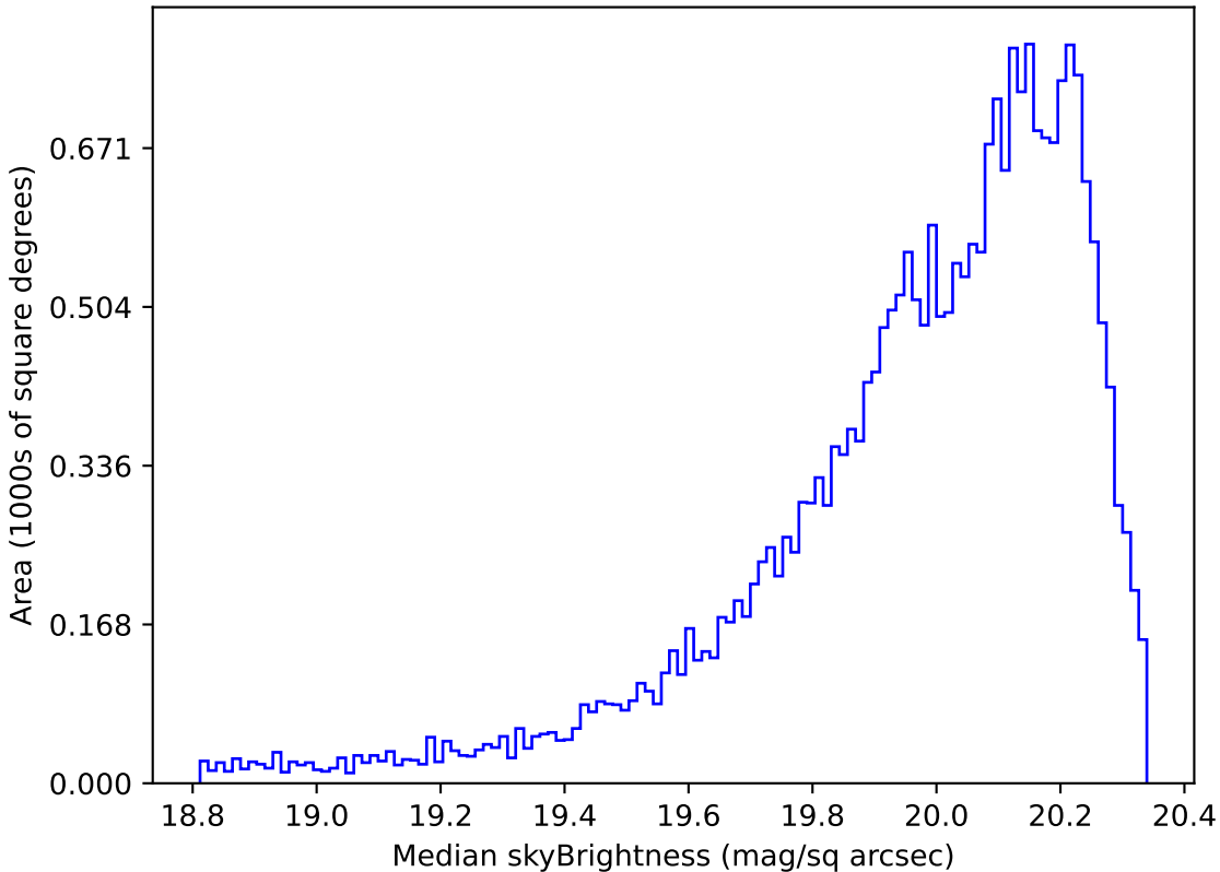
too_combined_s0.5_v3.4_10yrs Yr 1 i band: Median skyBrightness
