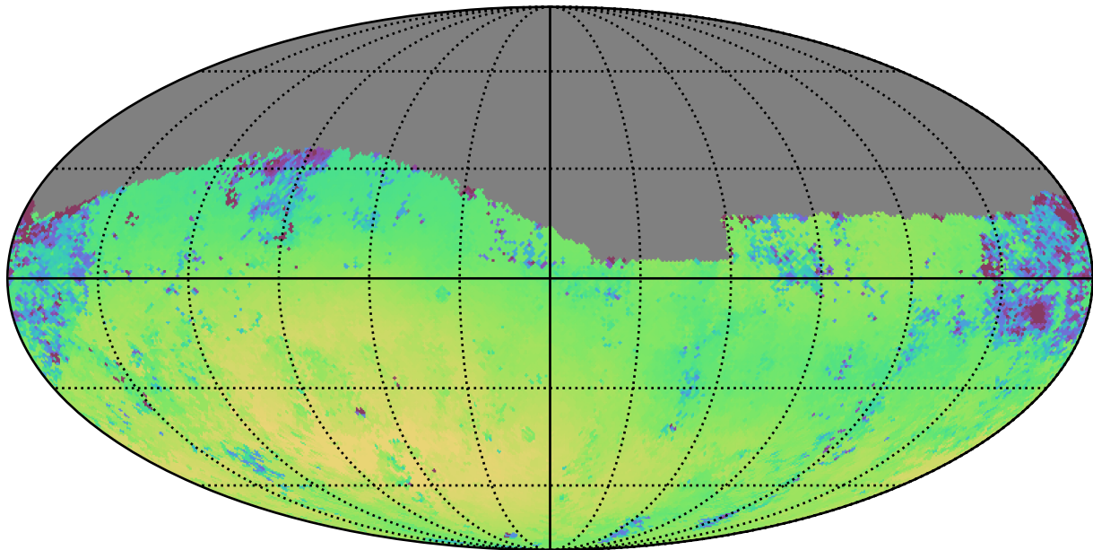
too_combined_s0.5_v3.4_10yrs Yr 1 g band: Median skyBrightness
