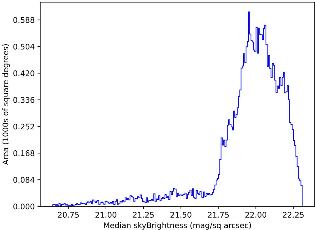
too_combined_s0.5_v3.4_10yrs Yr 1 g band: Median skyBrightness
