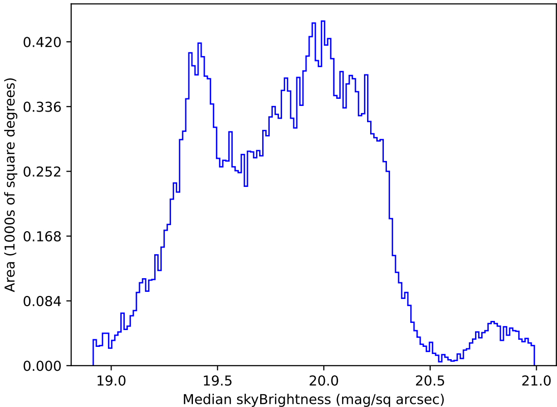
too_combined_s0.5_v3.4_10yrs Yr 1 all bands: Median skyBrightness
