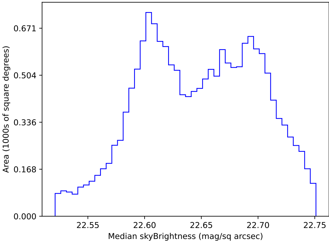
too_combined_s0.5_v3.4_10yrs WFD u band: Median skyBrightness
