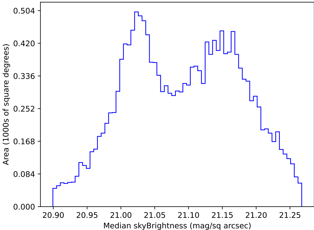
too_combined_s0.5_v3.4_10yrs WFD r band: Median skyBrightness
