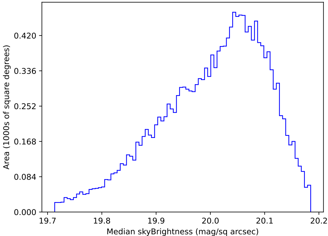
too_combined_s0.5_v3.4_10yrs WFD i band: Median skyBrightness
