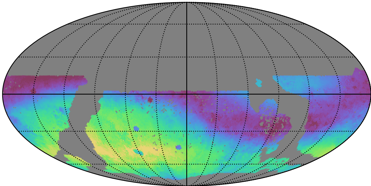
too_combined_s0.5_v3.4_10yrs WFD g band: Median skyBrightness
