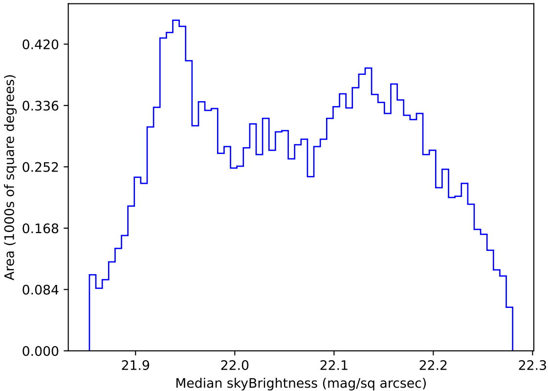
too_combined_s0.5_v3.4_10yrs WFD g band: Median skyBrightness
