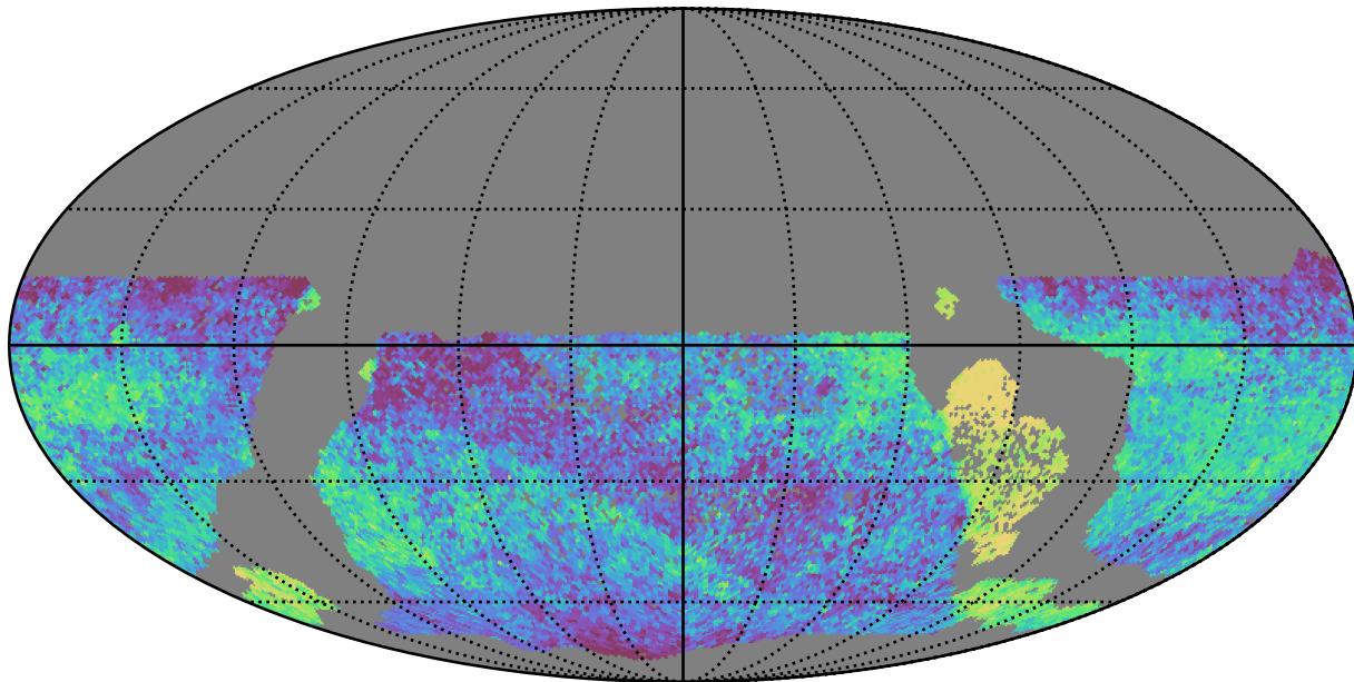
too_combined_s0.5_v3.4_10yrs WFD all bands: Median skyBrightness
