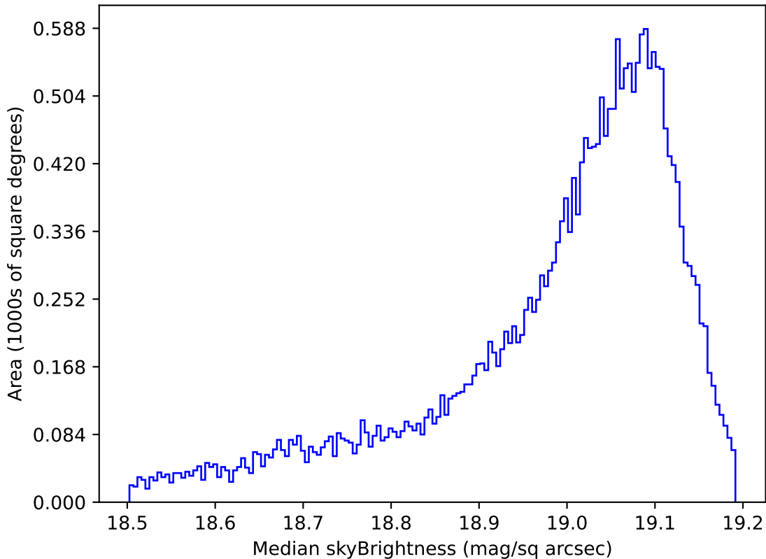
too_combined_s0.5_v3.4_10yrs All sky z band: Median skyBrightness
