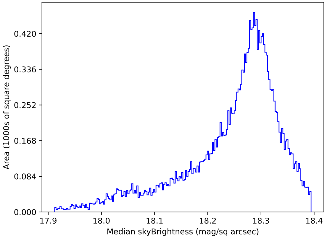
too_combined_s0.5_v3.4_10yrs All sky y band: Median skyBrightness
