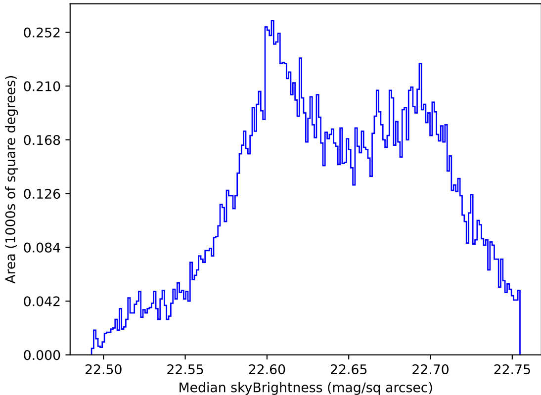
too_combined_s0.5_v3.4_10yrs All sky u band: Median skyBrightness
